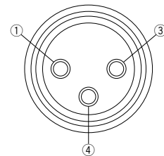
Connector's pin assignment for the input device connection (M8, 3 pins, socket)
