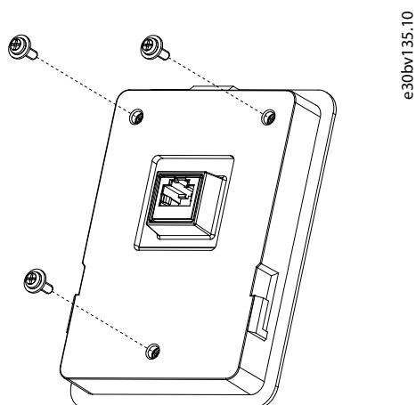
Illustration 3: Tightening Screws
