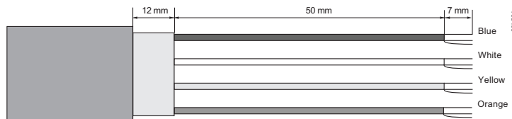
Figure 4-1 Cable end
